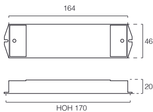
Receiver (S3.10.0422)
