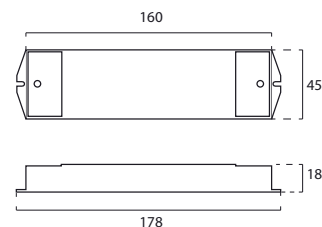
Receiver (S3.10.0276)
